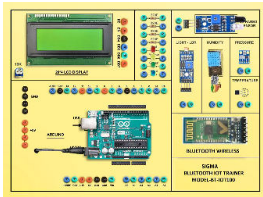
Transmitter
